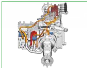
ON DEMAND 90L/MIN HYDRAULIC SYSTEM WITH 3 SETS OF REMOTES AND FLOW CONTROL
